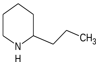
Conine
