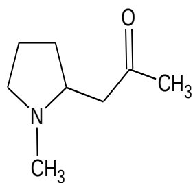
Hygrine
