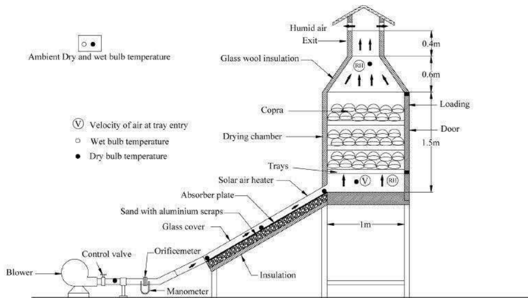
Figure 2.2.2.1: Layout of an Indirect Active Solar Dryer system
