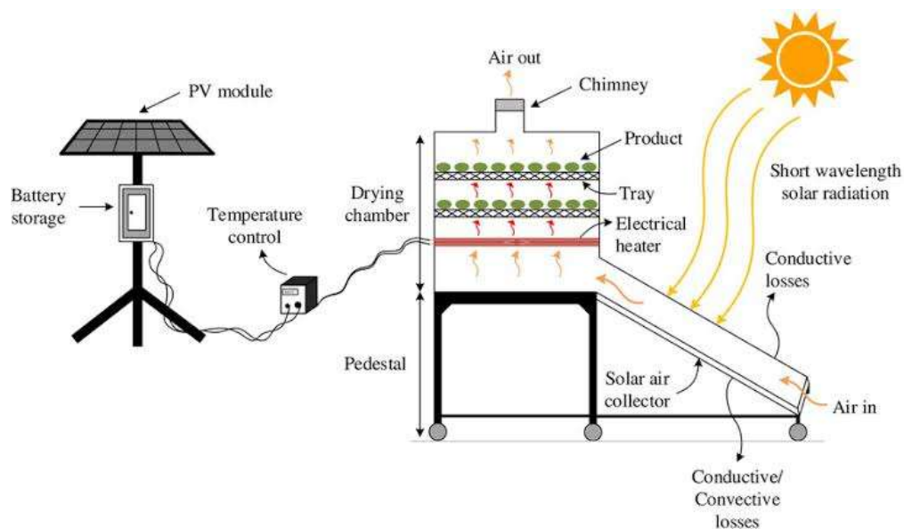
Figure 2.5.1: Working Principle of a Hybrid Solar Dryer
