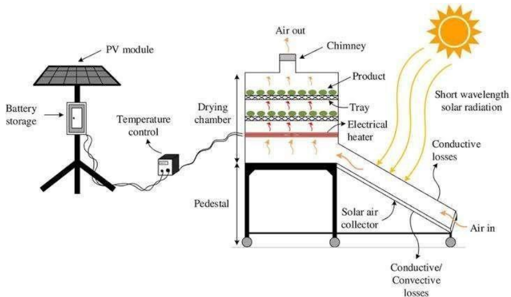
Figure 2.3.1: Working Principle of a Hybrid Solar Dryer
