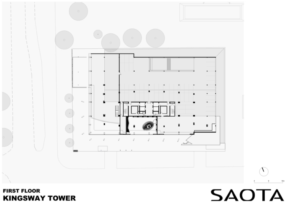
FIG3.3:- FIRST FLOOR PLAN
