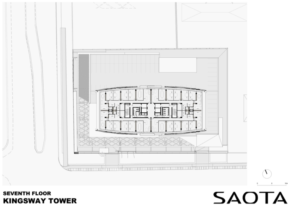
FIG 3.4:- SEVENTH FLOOR PLAN
