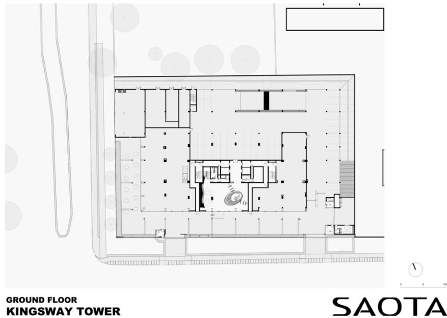
FIG 3.2:- GROUND FLOOR PLAN
