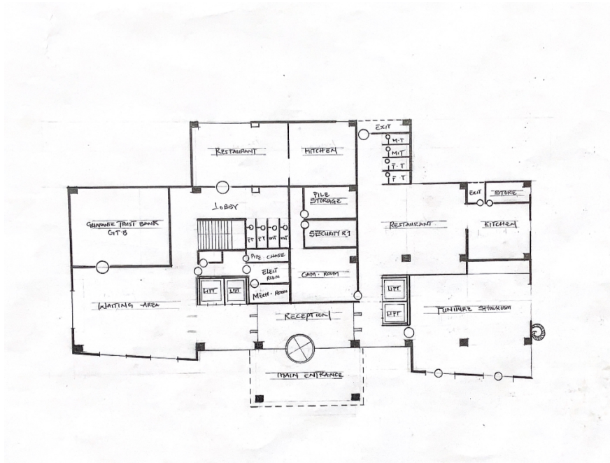
FIG 3.5:- FLOOR PLAN
