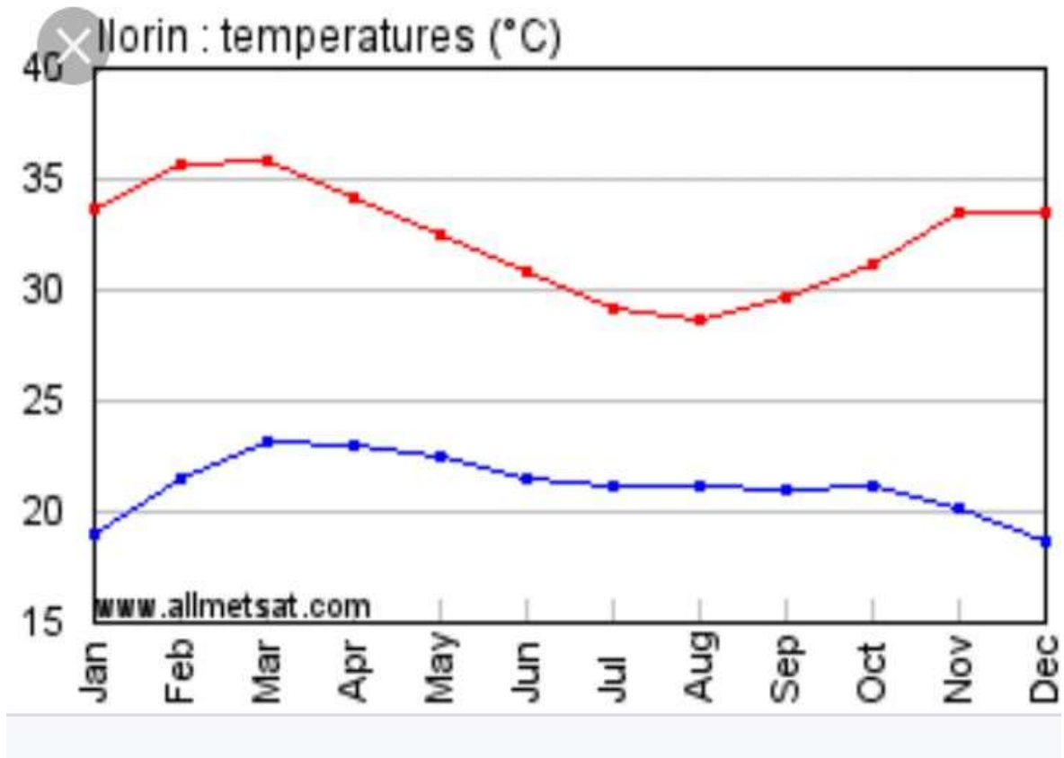
Figure 4.6: Graph of temperature in Ilorin
