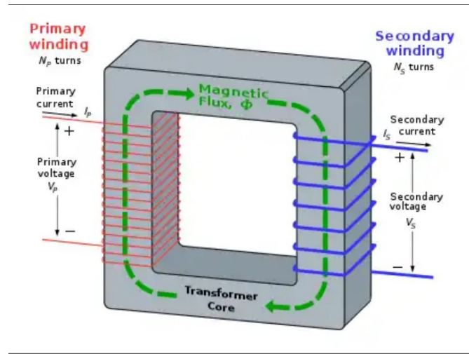
Fig. 2.5 Transformer winding
