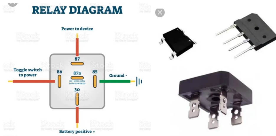
Fig.2.12 Relay
