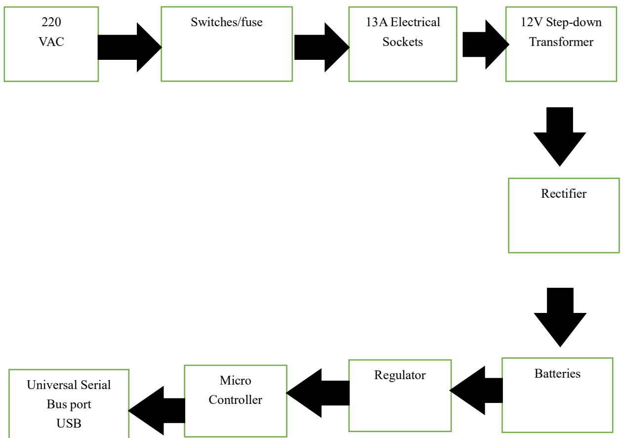
Fig. 3.1 Block diagram of the project
