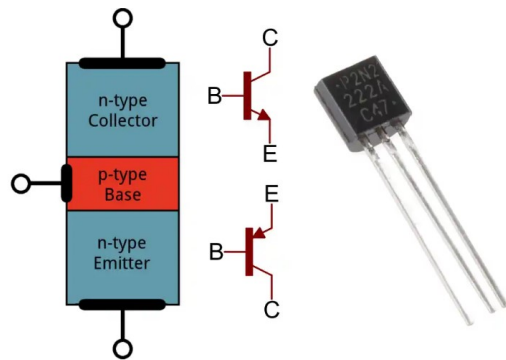
Fig.2.13 Transistor
