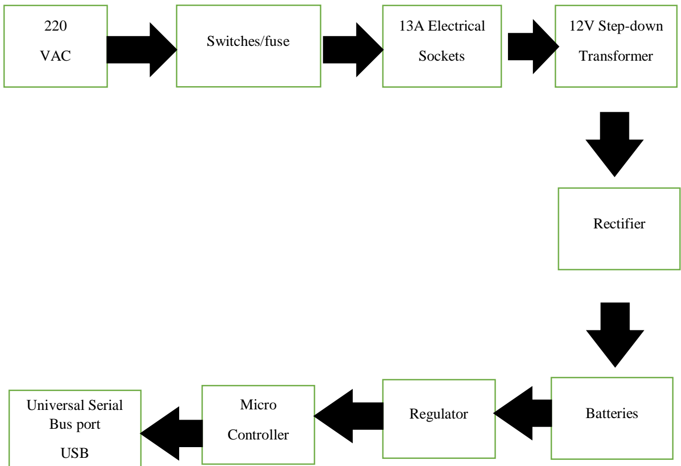
Fig. 3.1 Block diagram of the project
