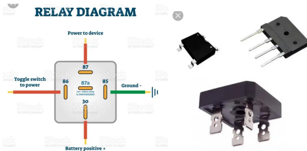
Fig.2.12 Relay
