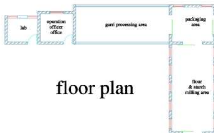
FIG 1.2:-FLOOR PLAN
