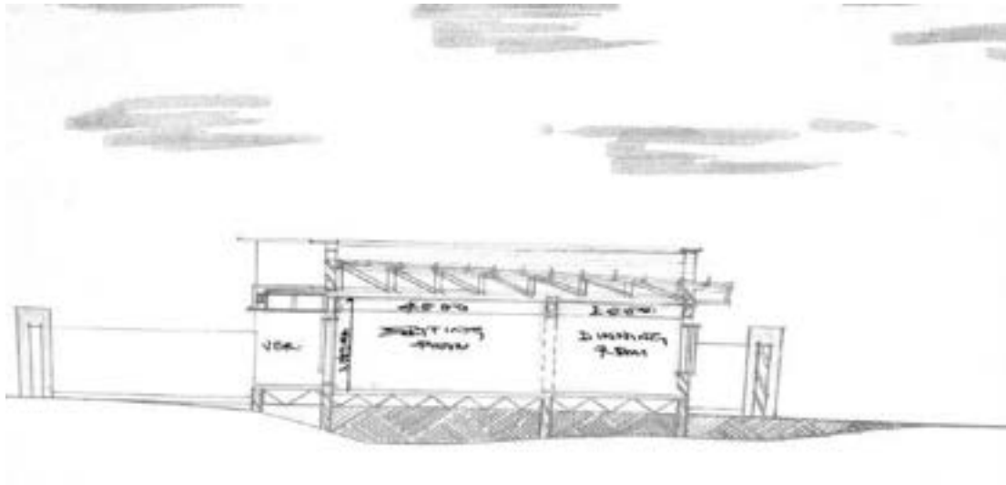
APPENDIX 15: SECTION FOR 1 BEDROM SEMI DETACHED BUNGALOW
