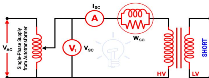
Figure 3.9: Short Circuit Test (Copper Loss Test)
