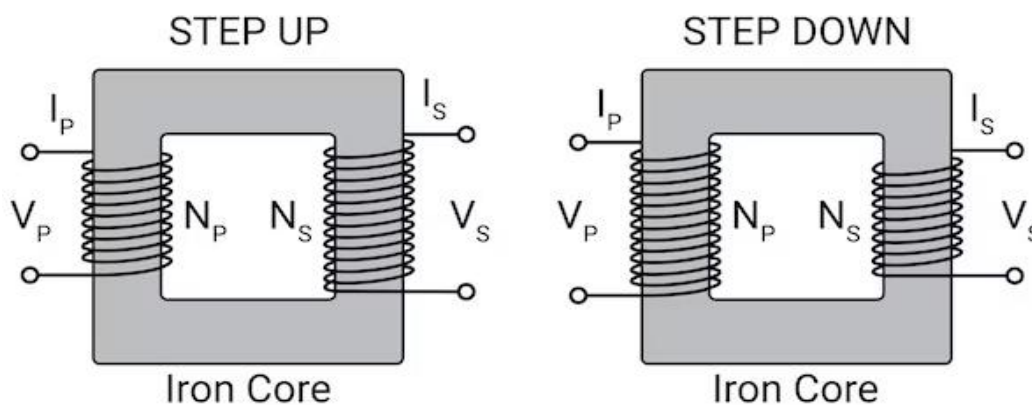
Figure 3.7: Circuit Diagram of Voltage Turn Ratio
