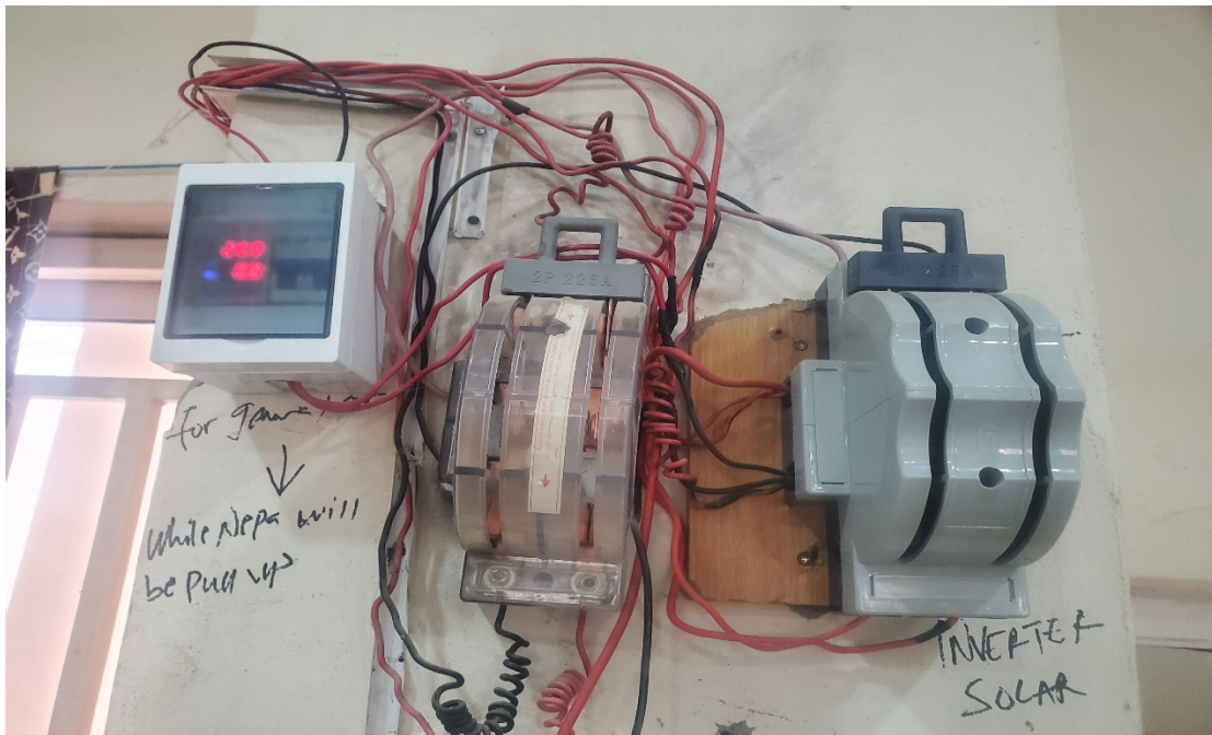
Figure 3.6: Changeover switch
