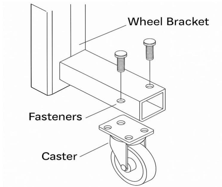
Figure 4.6.4 Shows structural frame reinforcement and wheel integration
