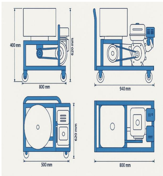
Figure 4.6.3 Front and side views with all key dimensions
