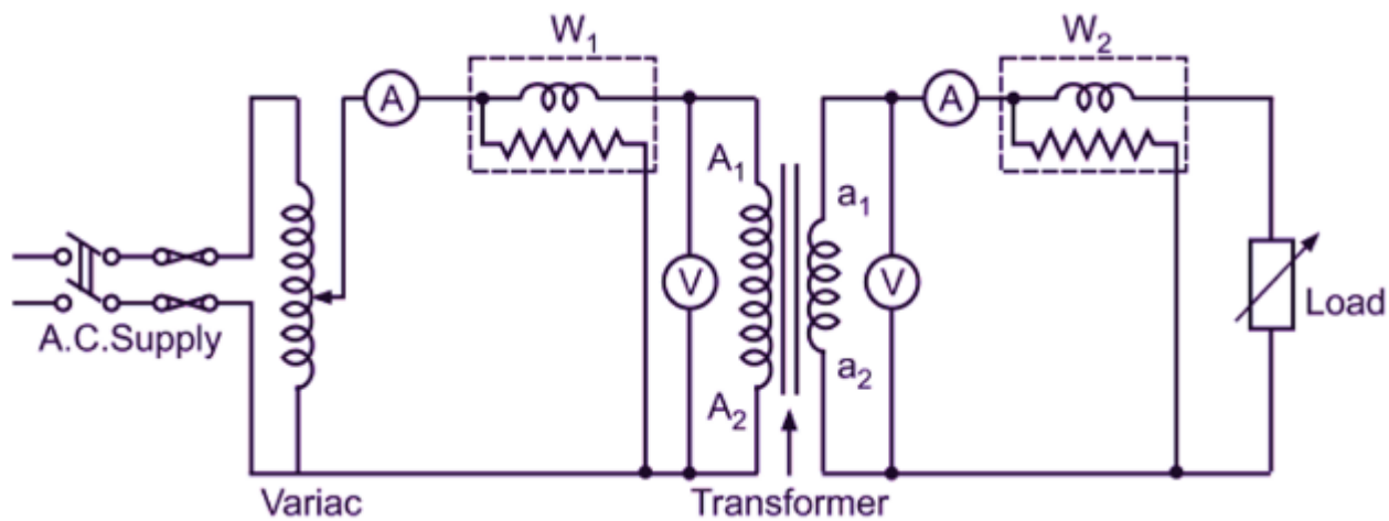
Figure 3.11: Circuit Diagram for Voltage Regulation
