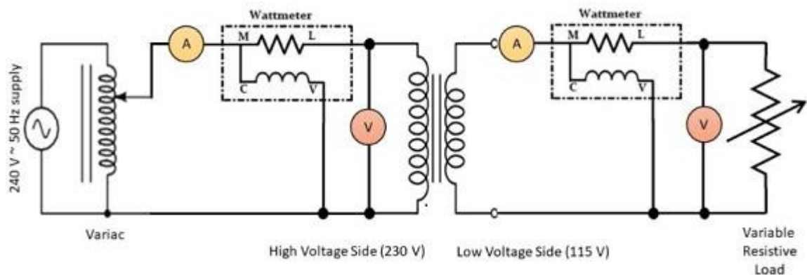
Circuit Diagram
