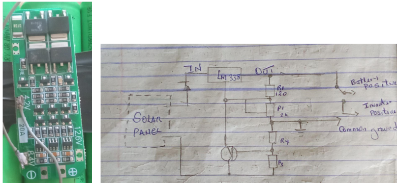
Figure 3.2 BMS CIRCUIT DIAGRAM AND IMAGE
