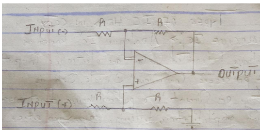
Fig 3.9: A simple analogue circuit diagram
