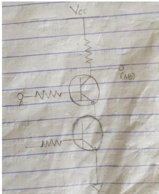
Fig 3.1.1: A simple digital circuit diagram is shown above
