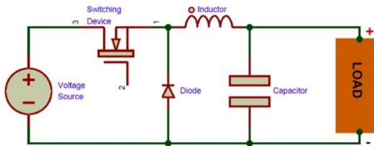
Figure4: thebuck convertercircuit
