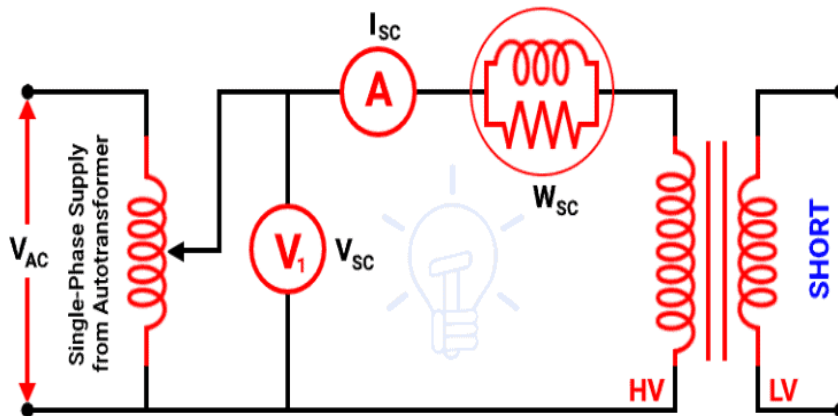
Figure 3.9: Short Circuit Test (Copper Loss Test)
