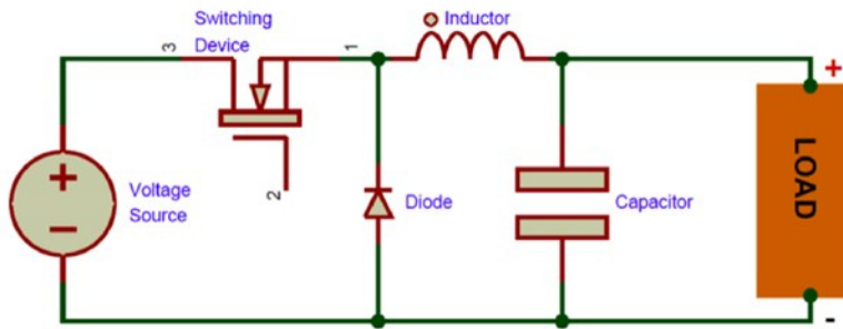
Figure 4: the buck converter circuit
