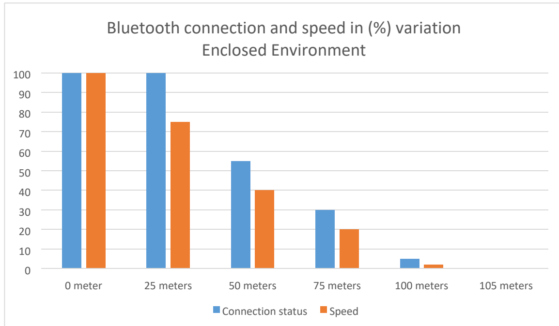
Figure 15: Bluetooth connection and speed in (%) variation in a enclosed environment
