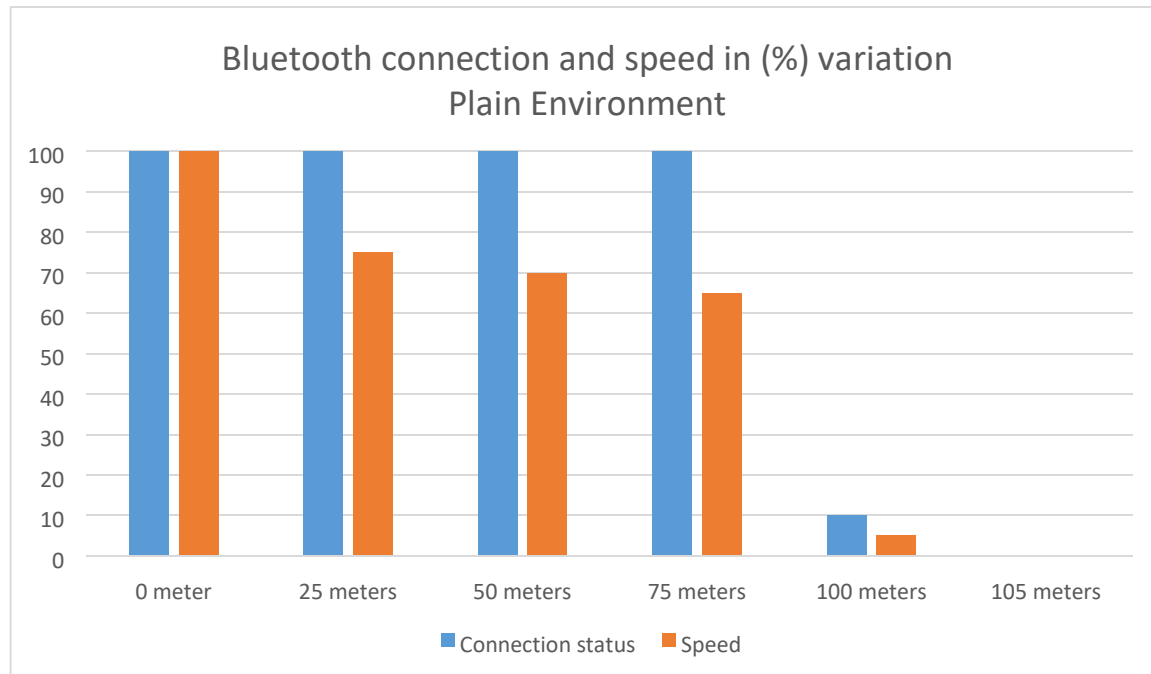
Figure14 Bluetooth connection and speed in (%) variation in a plain environment
