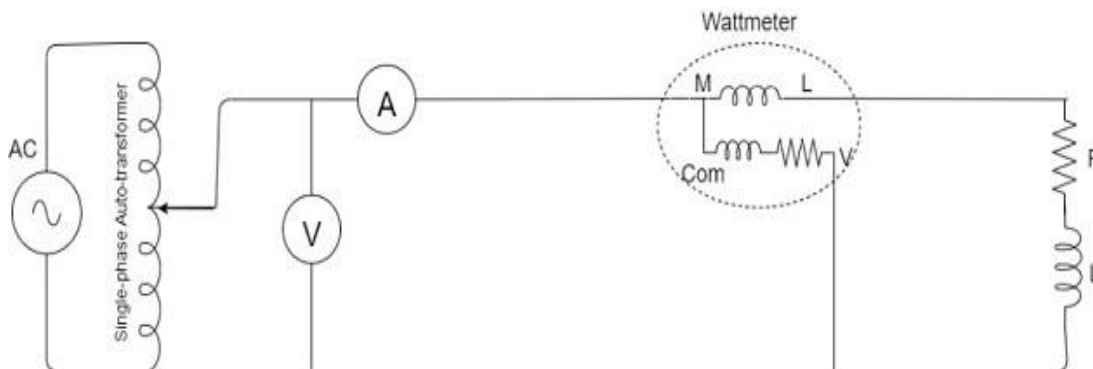
FIGURE 4.1- CIRCUIT DIAGRAM OF RLC CIRCUIT TRAINER
