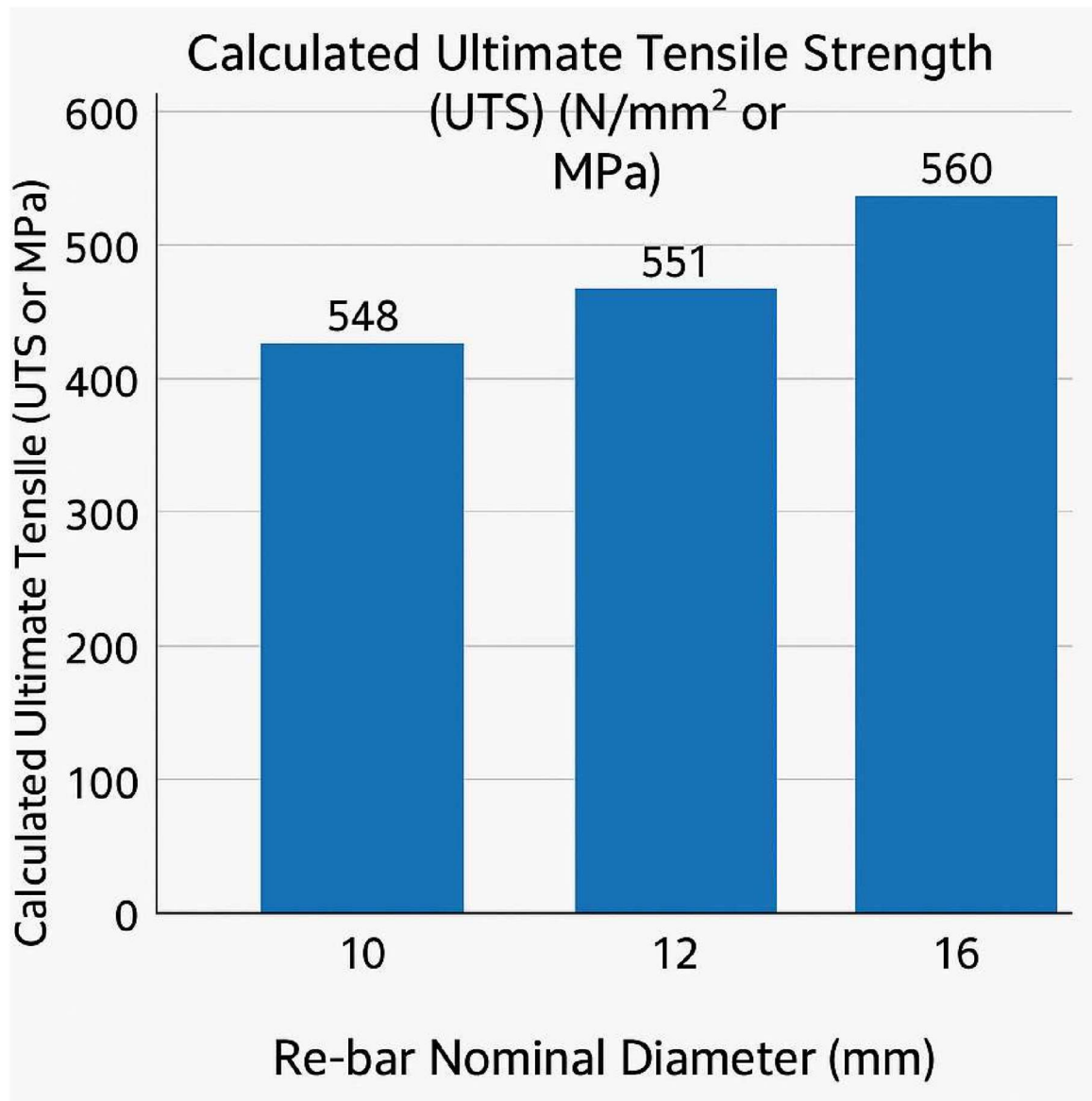
Figure 4.1: Comparative Ultimate Tensile Strength of KAM Industries Re-bars by Nominal Diameter
