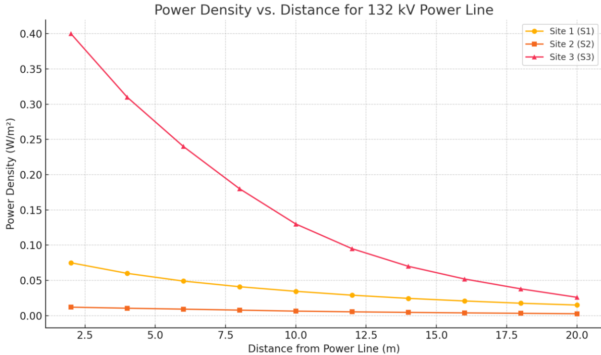
Figure 4.3 Power density measured from three different sites with 132 kV power line.
