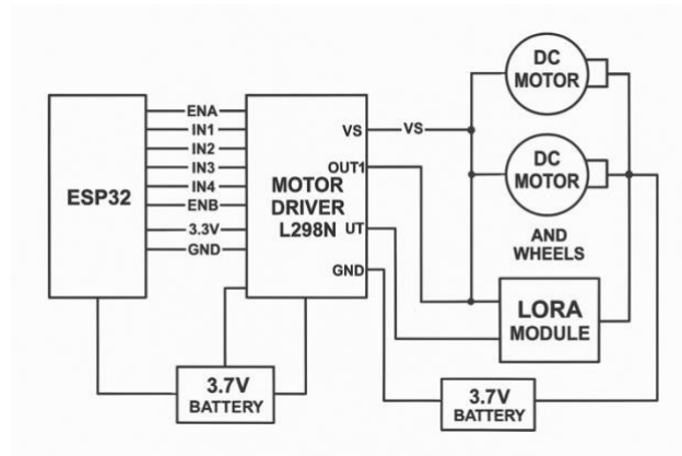
Figure 3.1: Circuit Diagram
