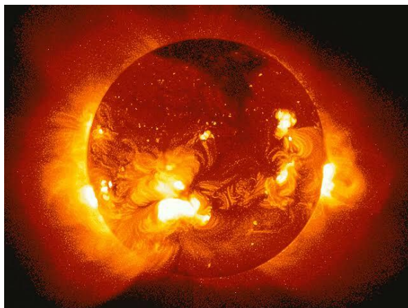
Figure 1. The structure of the sun (NASA)
