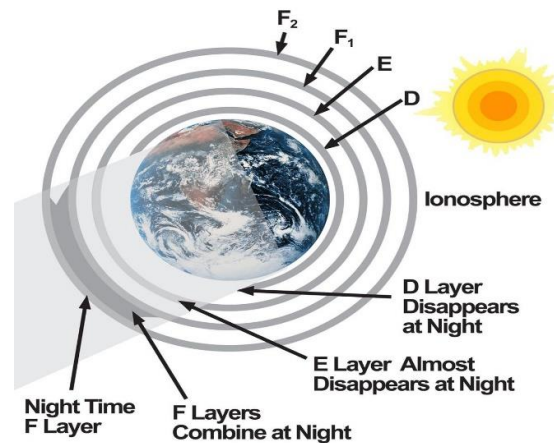
Fig 2.2: Layers of the ionosphere (Kelley, 2006)
