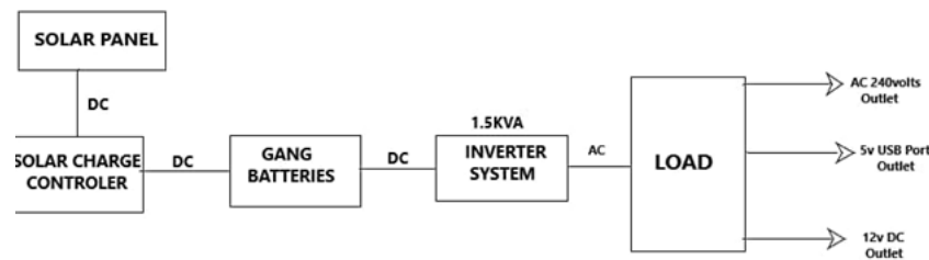
Figure 2.1: The Block Diagram of 1.5 kVA Mobile Inverter System
