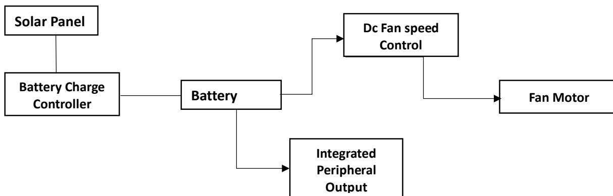
Figure 3.1 Assembling block diagram
