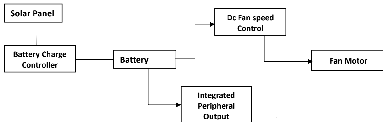
Figure 2.12 Assembling block diagram
