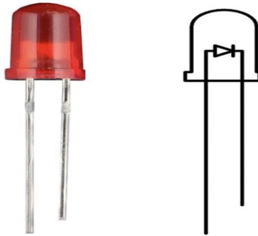
Figure 2.7: Miniature LED
