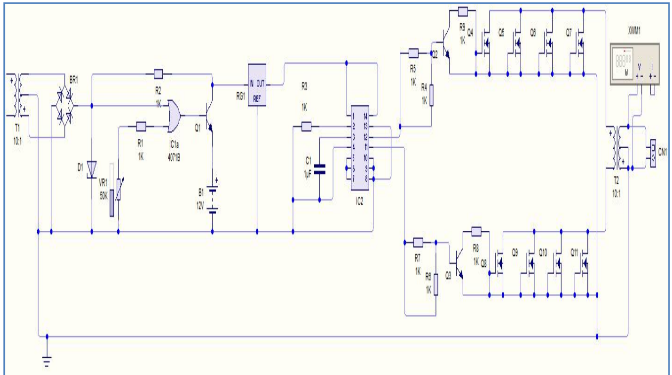
Figure 3.1 Circuit Diagram for 2KVA Mobile Inverter Systems.
