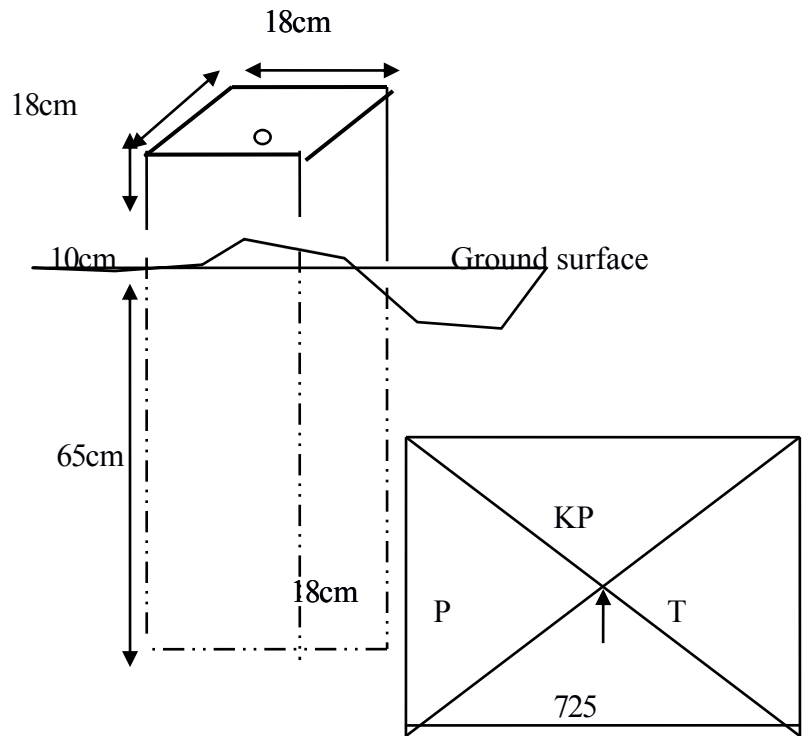
Figure 3.2.1: Plan View
