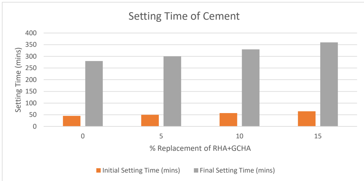
Figure 4.5: Setting Time Against % Replacement of RHA+GCHA
