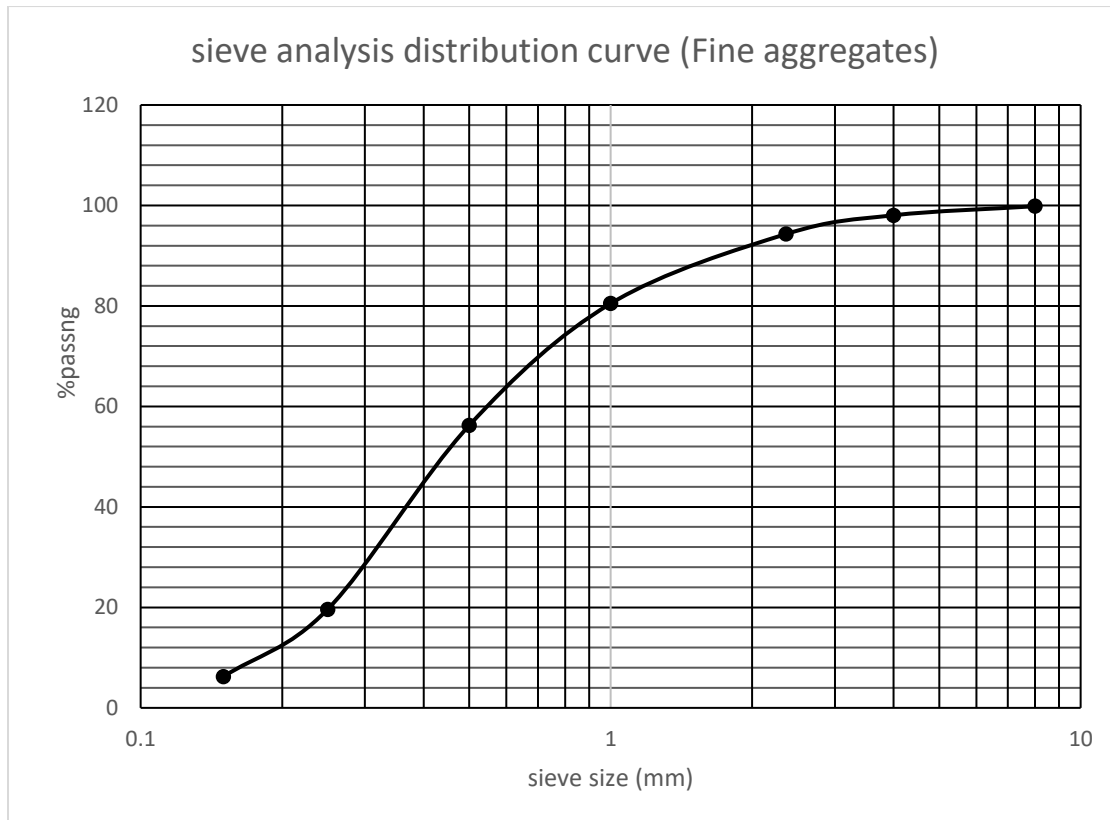
Figure 4.1: %Passing Against Sieve Sizes for Fine Aggregates
