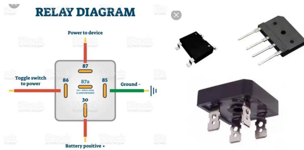
Fig. 2.8 Relay
