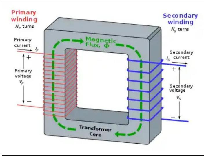
Fig. 2.5 Transformer winding
