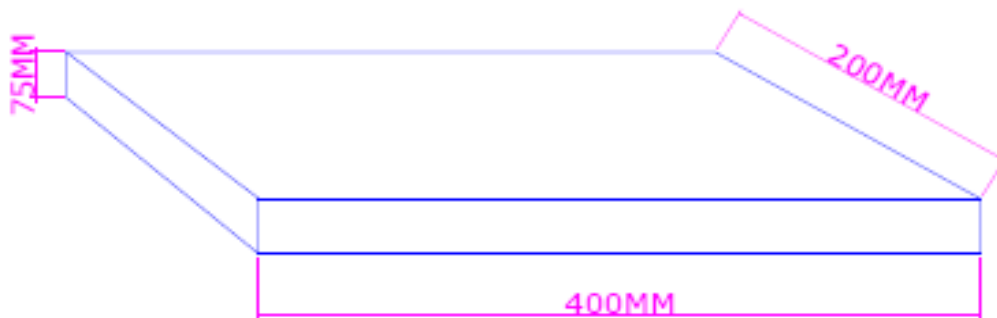
Figure 3.1: Concrete Slab Section.
