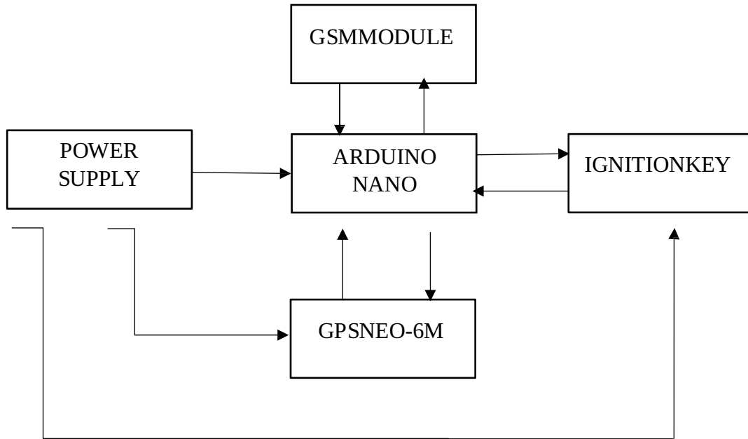
Fig.3.1:Block Diagram
