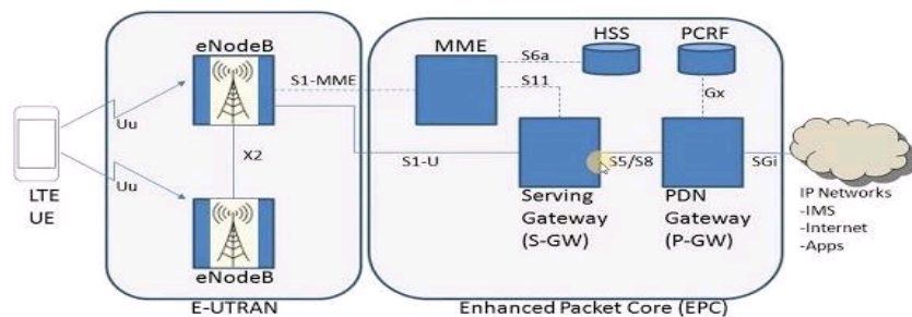
Fig2.6:LTEand4Gnetwork
