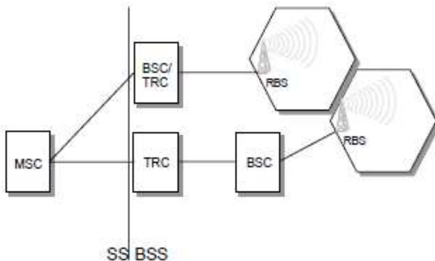
Figure 1 BSS in Ericsson's GSM systems.
