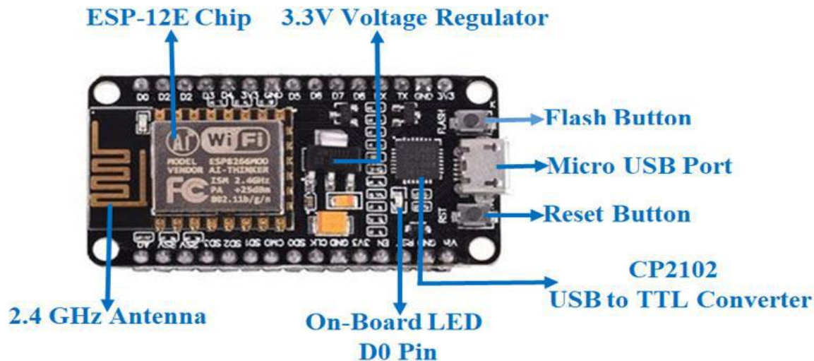
Figure 4.5: ESP8266/NodeMCU
