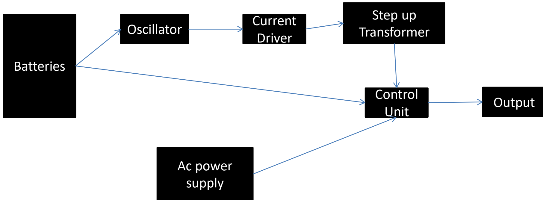
Figure 4: The Block Diagram of the Proposed 2.5 kVA Inverter System
