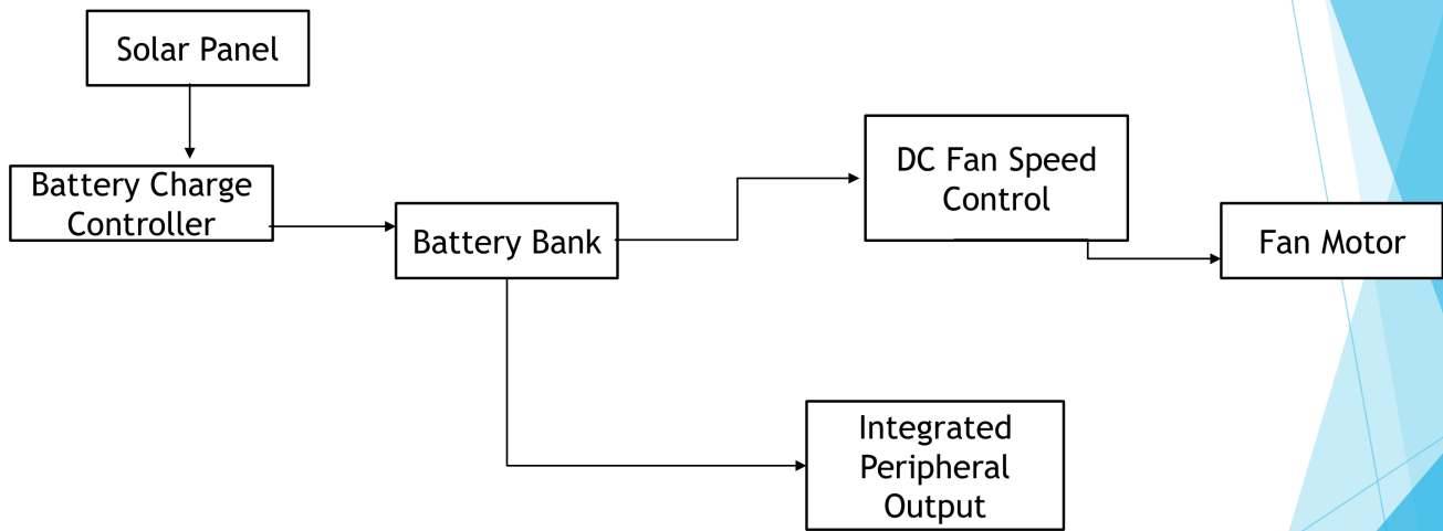
Figure 3: The Block Diagram of a Proposed 10 Watts Solar Powered DC Standing Fan
