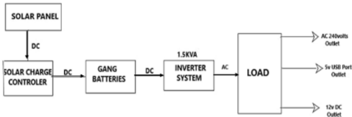
Figure 3: The Block Diagram of 1.5 kVA Mobile Solar Inverter System
