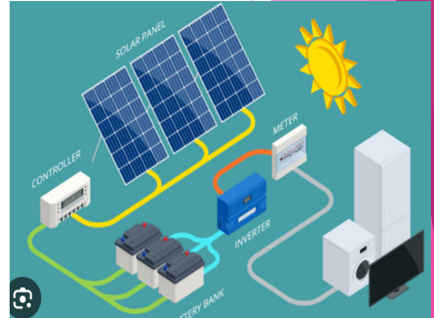
Figure 1: Standalone Inverter System
