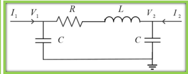
Figure 1: Transmission Line RLC model
