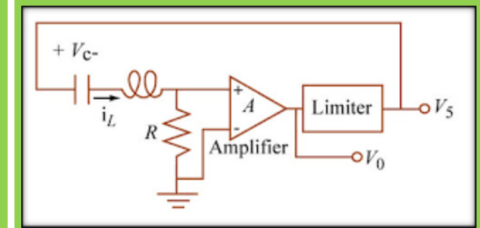
Figure 2: RLC Oscillator model
