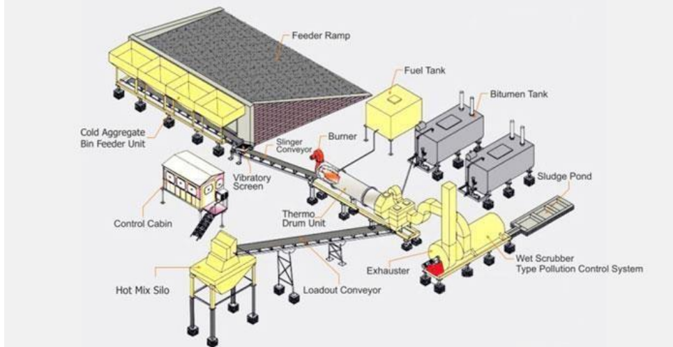
General layout of Asphalt drum mix plant
