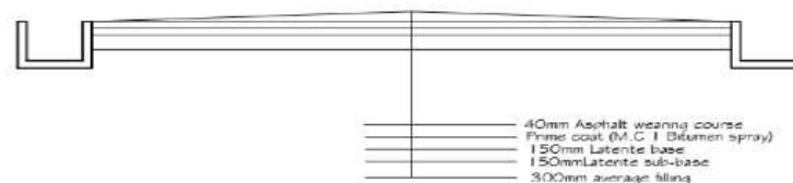
Plate 1.0: Road cross section
