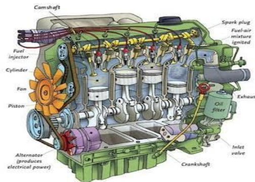
INTERNAL COMBUSTION ENGINE
