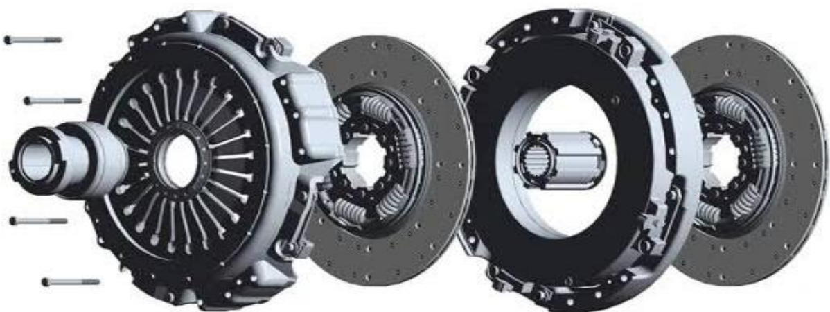
CLUTCH COMPONENT
