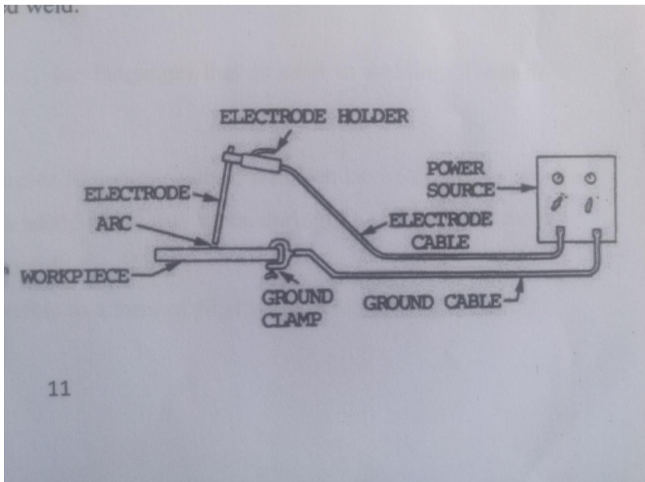
FIG.5: ARC WELDING
